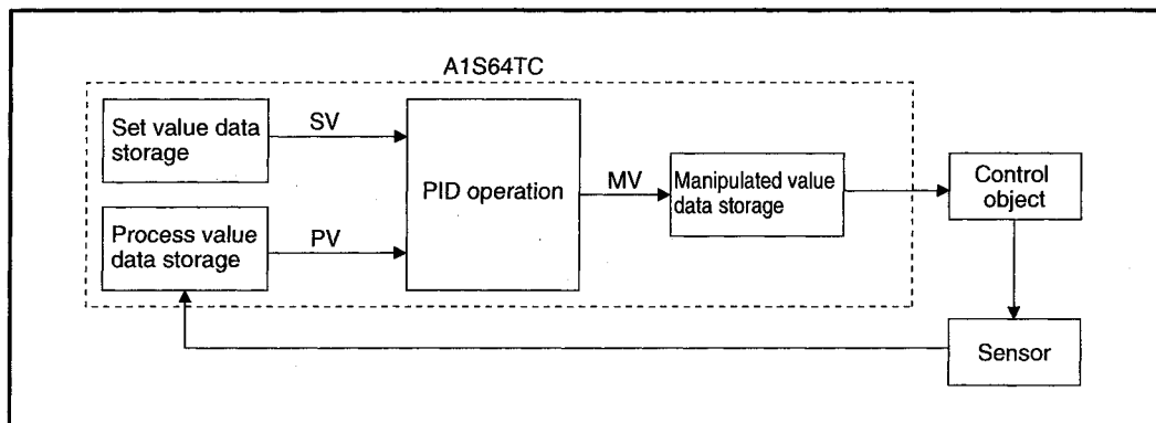
Fig. 1.3 The PID control system
