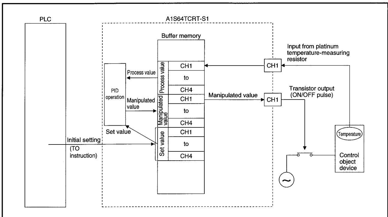
Fig. 1.1 A1S64TCRT-S1 processing overview
