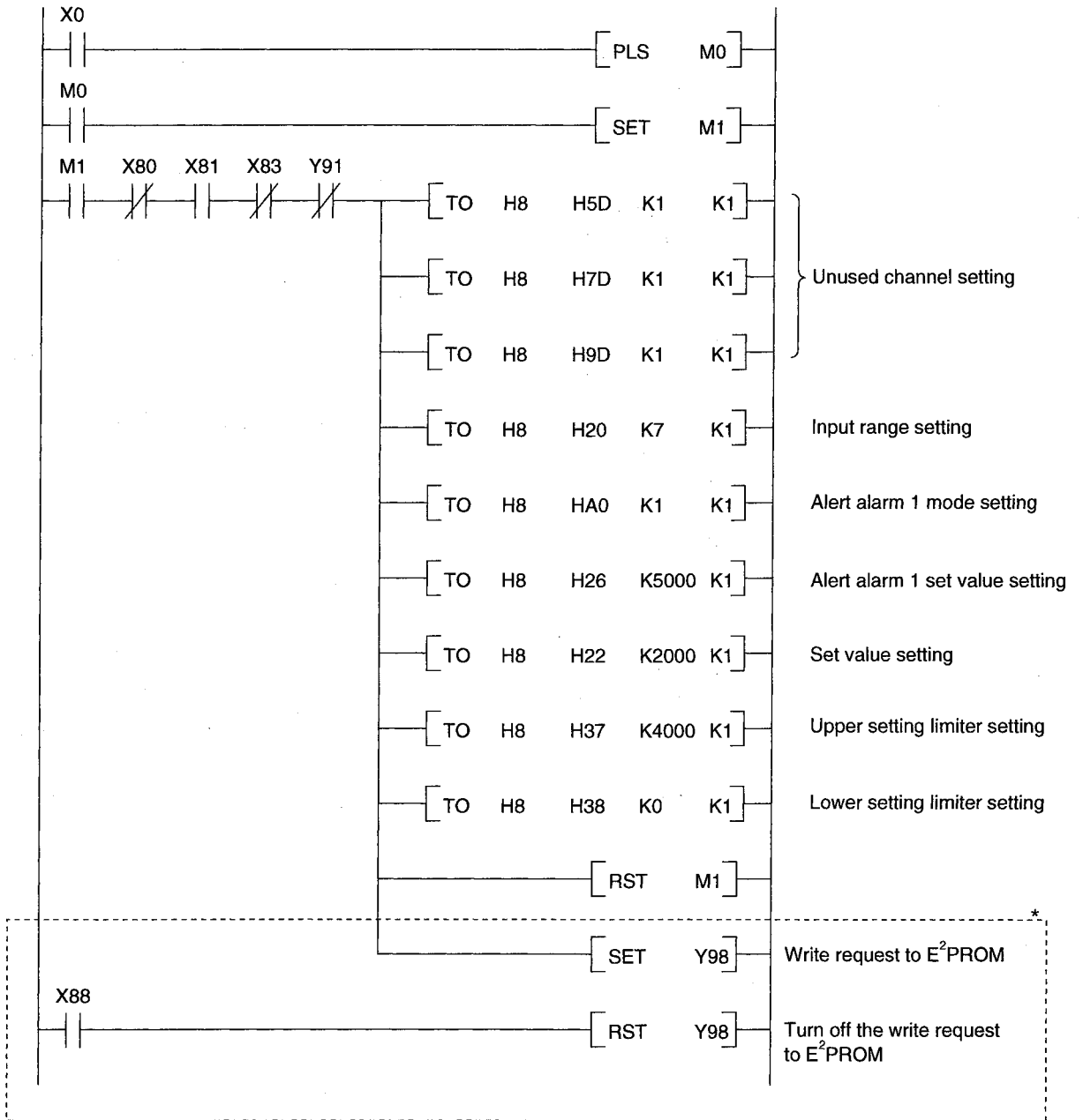
(b) Unused channel, input range, alert alarm 1, and set value, upper/lower setting limiter setting
