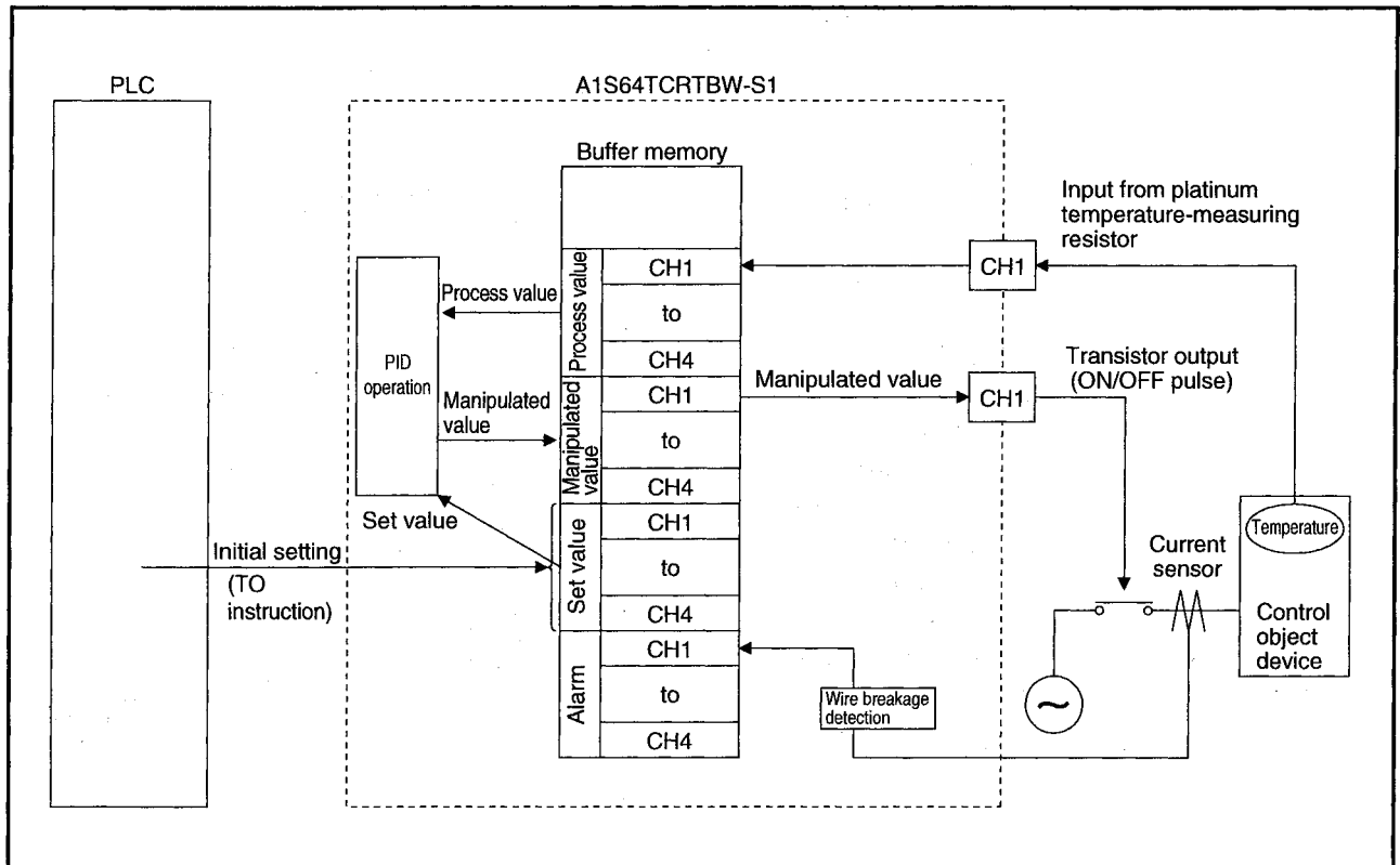
Fig. 1.2 A1S64TCRTBW-S1 processing overview
