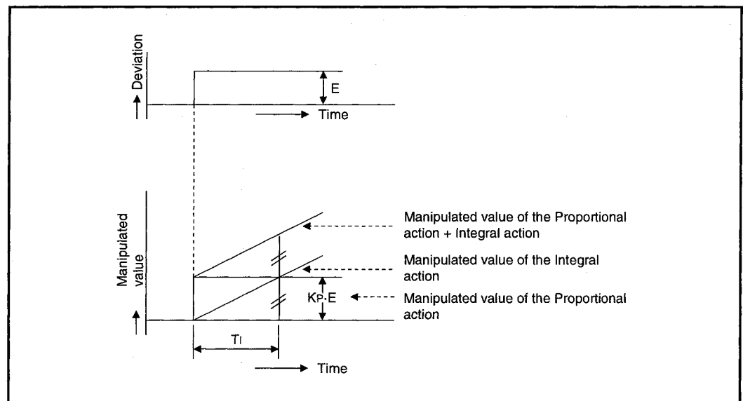
Fig. 1.9 Integral action for step response
