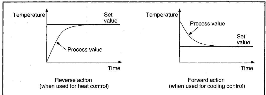
Fig. 1.7 Process control example in reverse action and forward action
