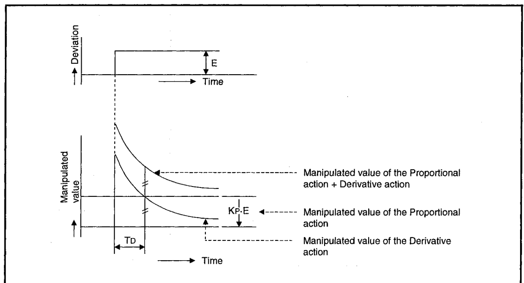
Fig. 1.10 Derivative action for step response
