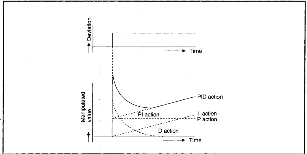
Fig. 1.11 PID action for step response
